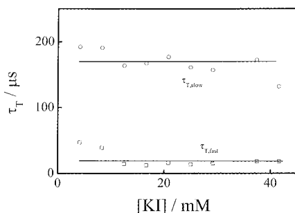
Figure 10. KI concentration dependence of lifetimes of fast and slow relaxations determined in Figure 9, where [ZnPc] = [PEO10000] = 0.2 mM.
